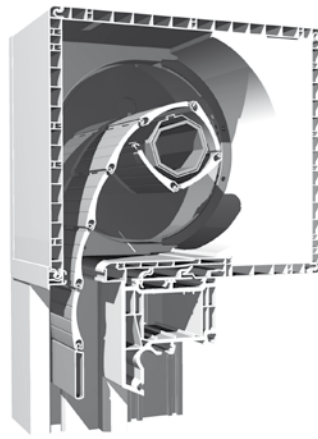
EasyBox (AK-E)
